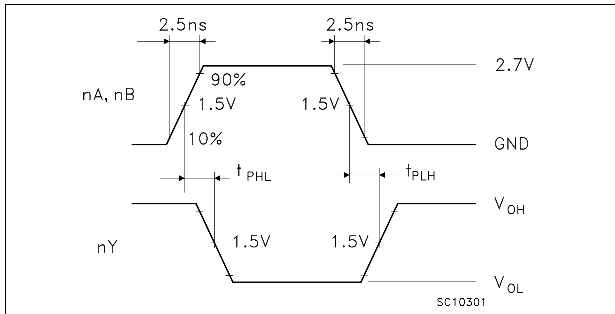
WAVEFORM : PROPAGATION DELAYS ( f=1\text{MHz} ; 50% duty cycle)
